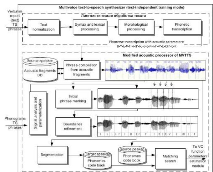
Figure 2. Text-independent training process in MVTTS
